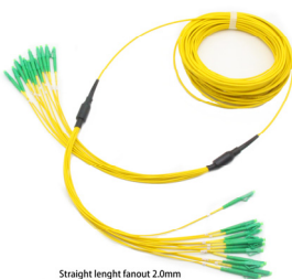
Straight length fanout 2.0mm 12x LC APC simplex
